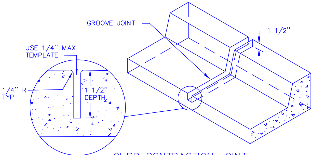
CURB CONTRACTION JOINT
