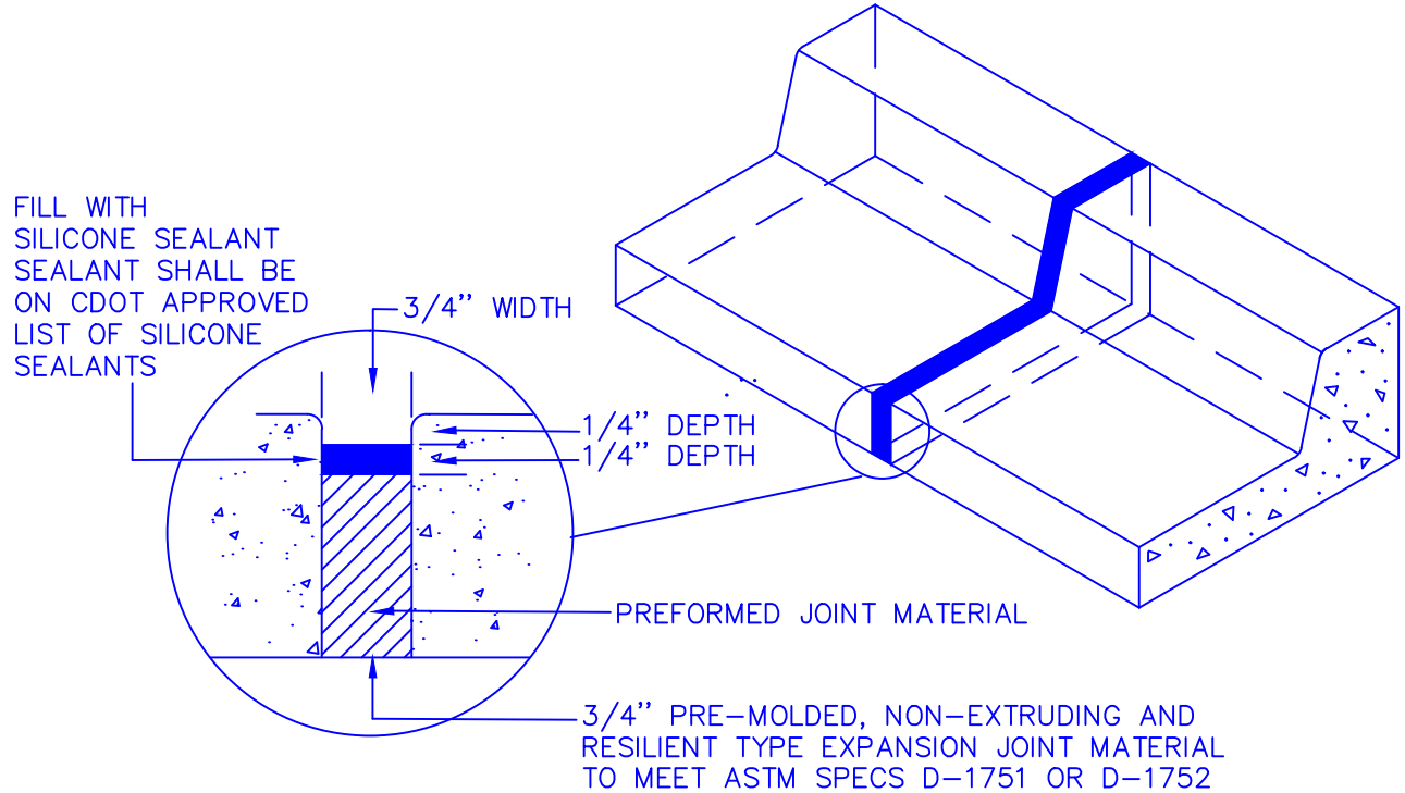
CURB EXPANSION JOINT
