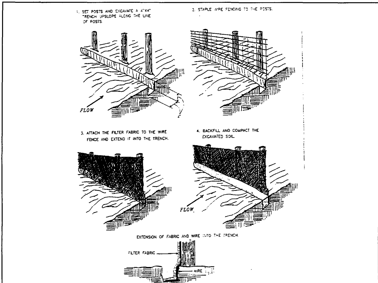
Figure 14: Construction of a silt fence
