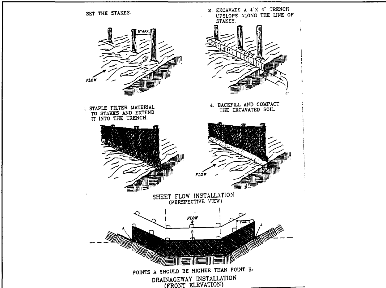
Figure 15: Construction of a silt fence (without wire support)
