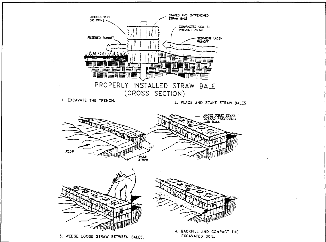
Figure 13: Construction of straw bale barrier
