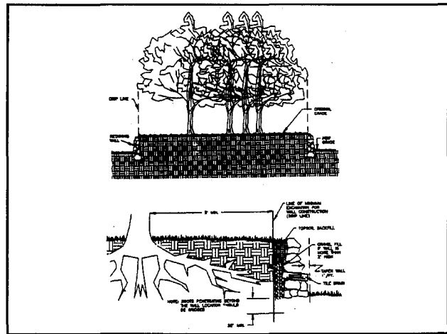
Figure 4: Tree wall
