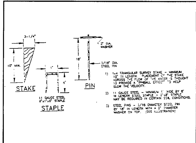
Figure 10: Stakes, staples and pins for installation of soil stabilization blanket.
