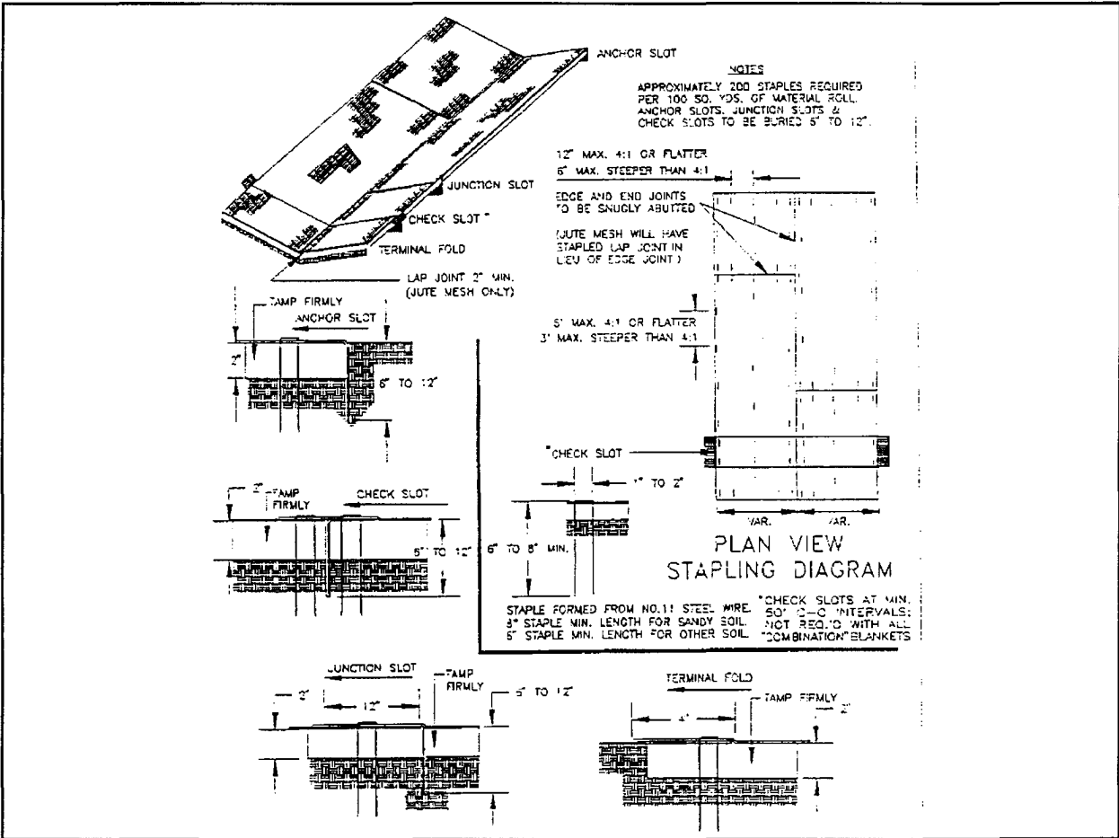
Figure 9: Typical treatment, soil stabilization blanket.
