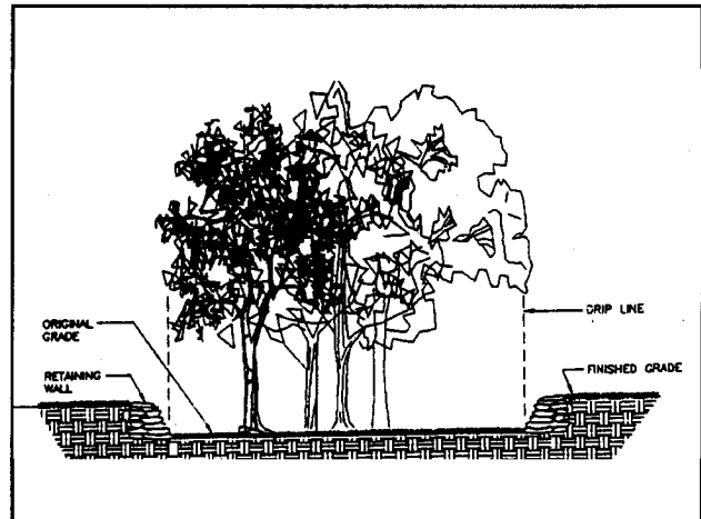
Figure 2: Tree Well
