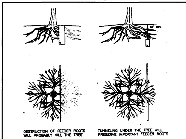
Figure 5: Trenching vs. tunneling
