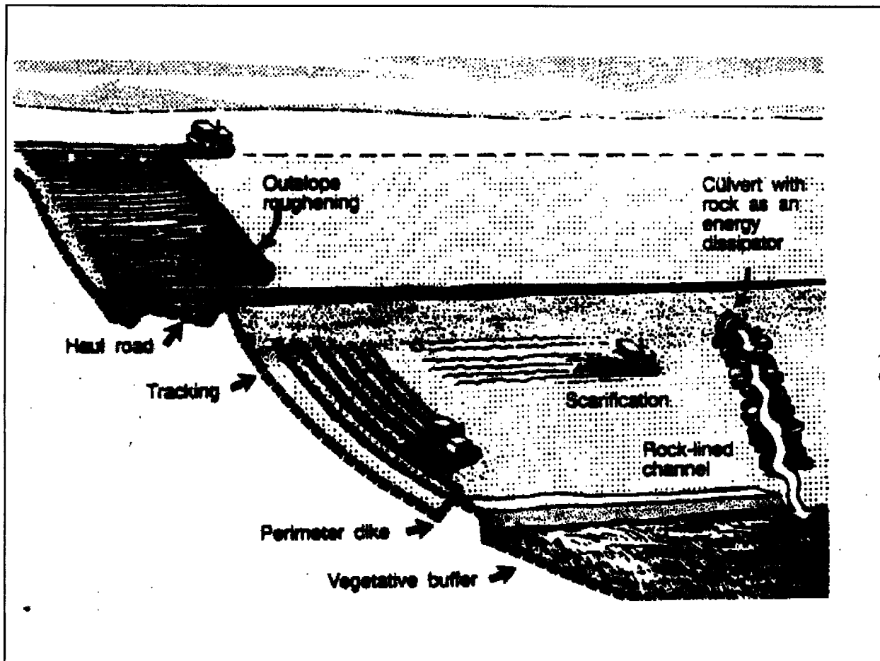
Figure 6: Surface Roughening
