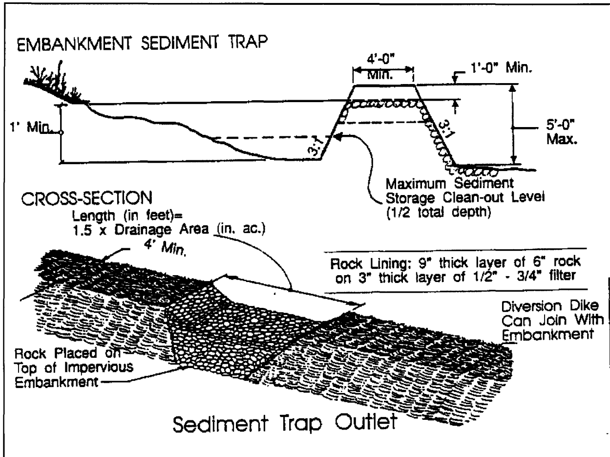
Figure 16: Temporary sediment trap
