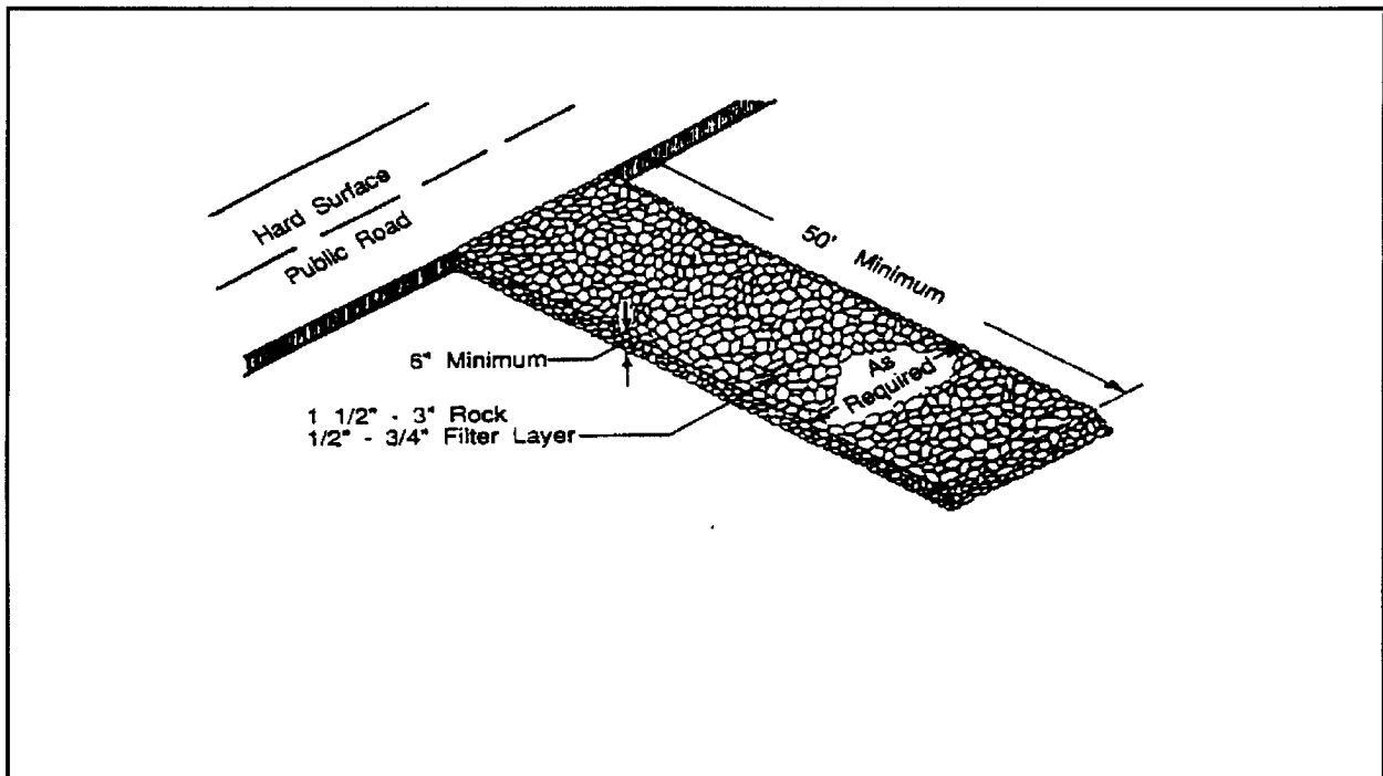
Figure 12: Detail of tracking control application
