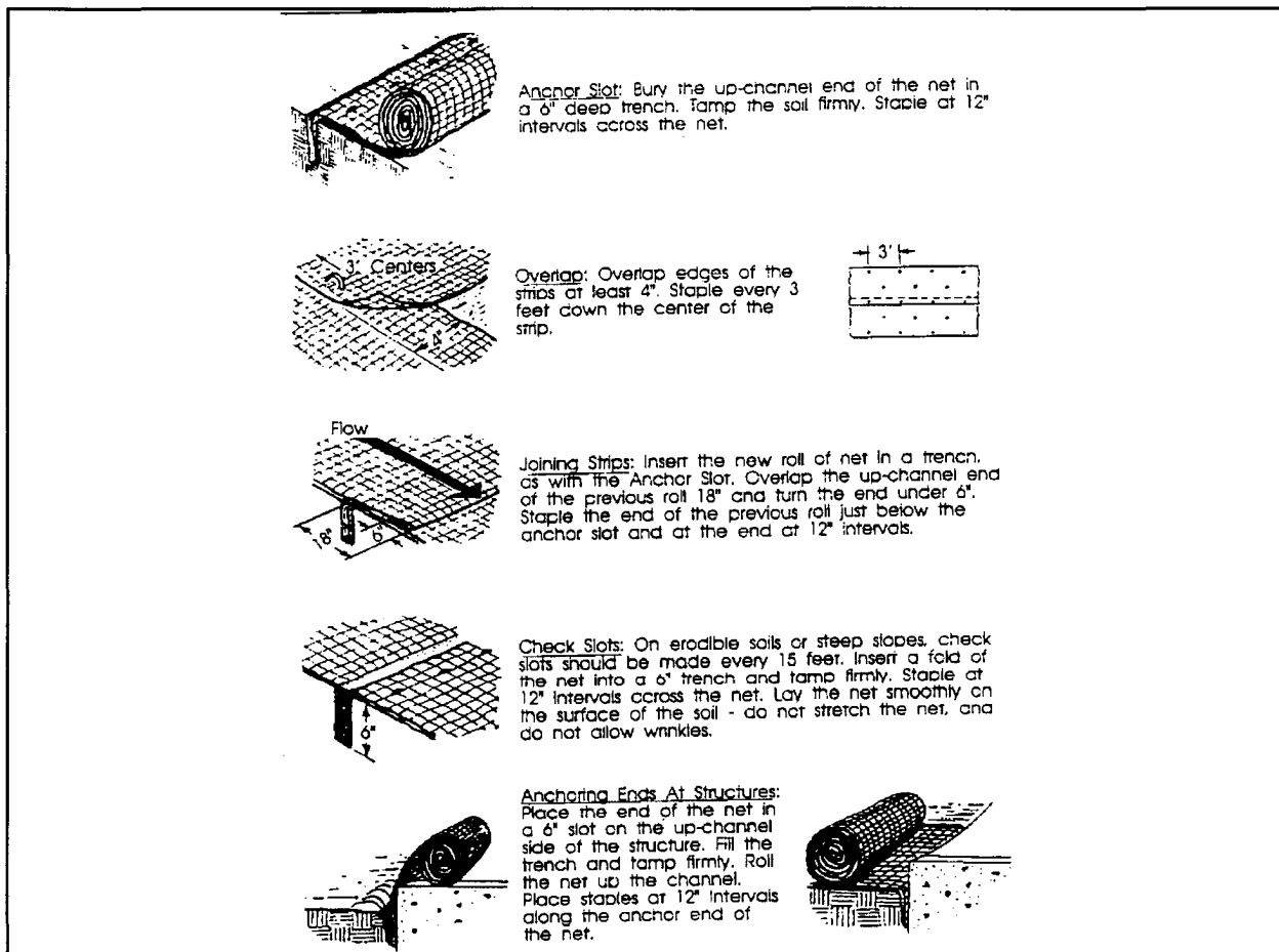
Figure 8: Installation of blankets, netting and matting.
