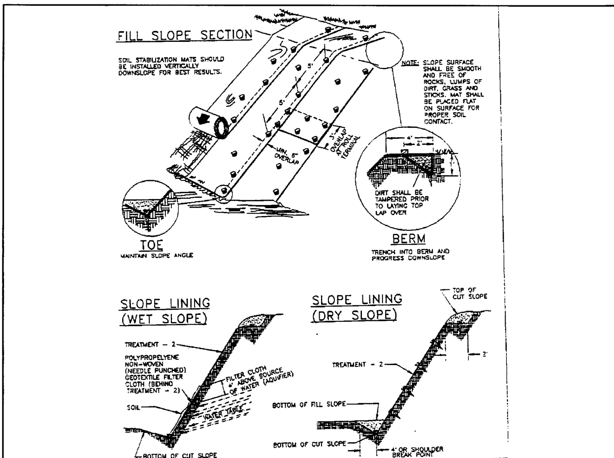
Figure 11: Soils stabilization matting, slope installation.
