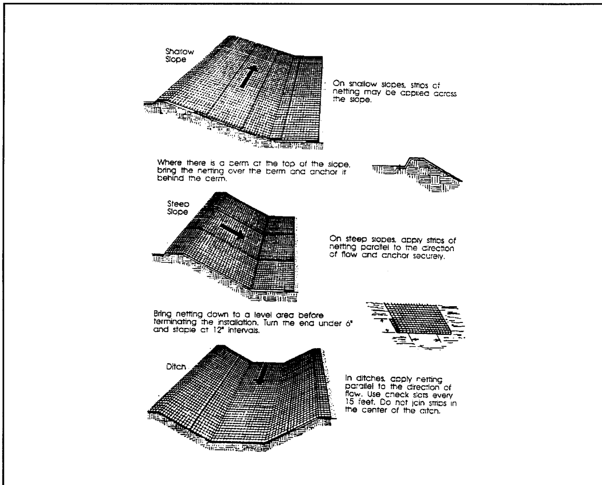
Figure 7: Typical orientation of soil stabilization blanket (treatment 1).
