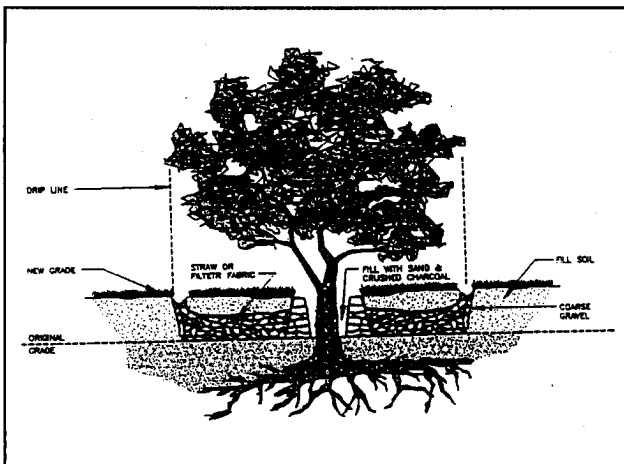
Figure 3: Tree well, alternate
