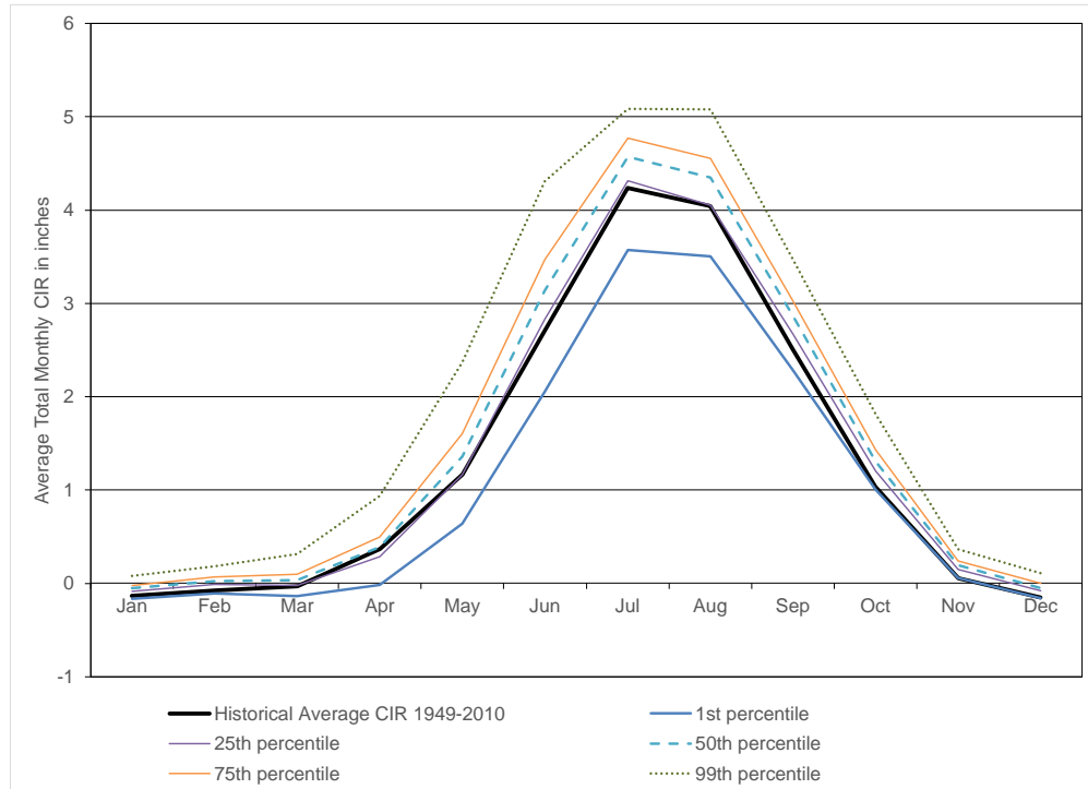
Figure 5-4: Range of Projected Average Monthly IWR with Climate Change for Boulder
