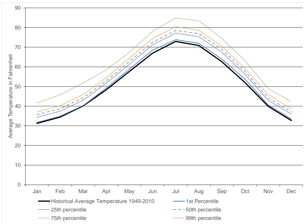
Figure 5-2: Range of Projected Average Monthly Temperature with Climate Change for Boulder, Year 2070
