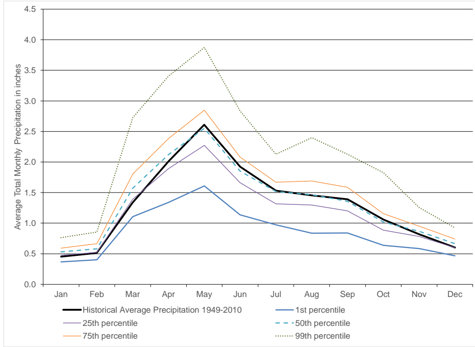
Figure 5-3: Range of Projected Average Monthly Precipitation with Climate Change for Boulder, Year 2070
